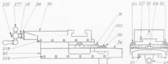
Fig. 19. Position of Compound Rest Parts in Assembly.
