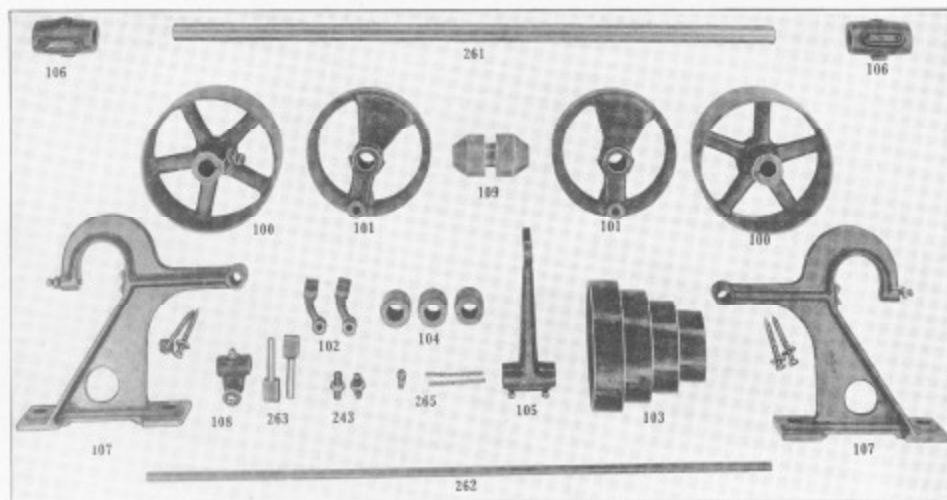
Fig. 25. Various Parts of Double Friction Countershaft.
