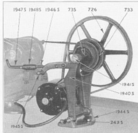
Fig. 32. Horizontal V-Belt Countershaft, with Belt Tension Adjustment.
