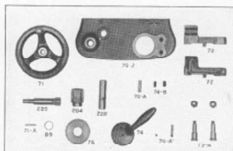
Fig. 12. Apron Parts for "Workshop" Lathe.
