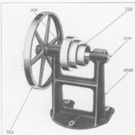
Fig. 31. Horizontal V-Belt Countershaft, Plain Type.
