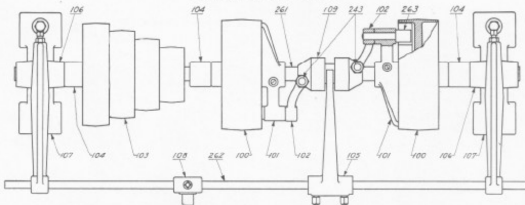
Fig. 28. Illustration Showing Parts of Double Friction Countershaft.
