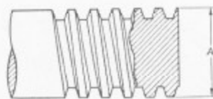
Acme Screw Thread.
