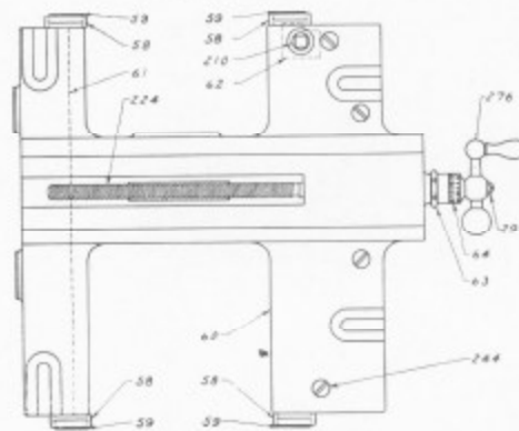
Fig. 18. Position of Saddle Parts in Assembly.
