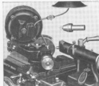
Fig. 41. Electric Grinder Mounted on Tool Post.
