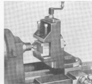
Fig. 42. Milling and Keyway Cutting Attachment for Lathe.
