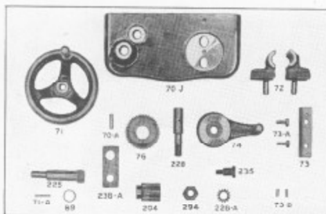
Fig. 11. Apron Parts for Toolmaker Lathe.
