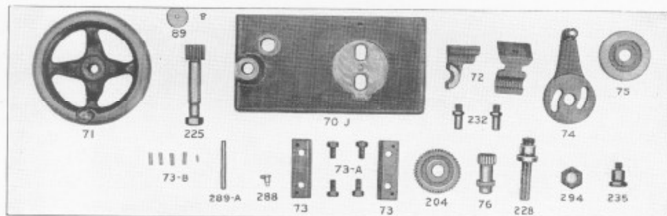
Fig. 10. Apron Parts for Junior South Bend Lathe.
