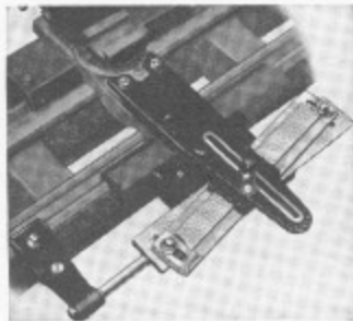
Fig. 40. Graduated Taper Attachment for Lathe.
